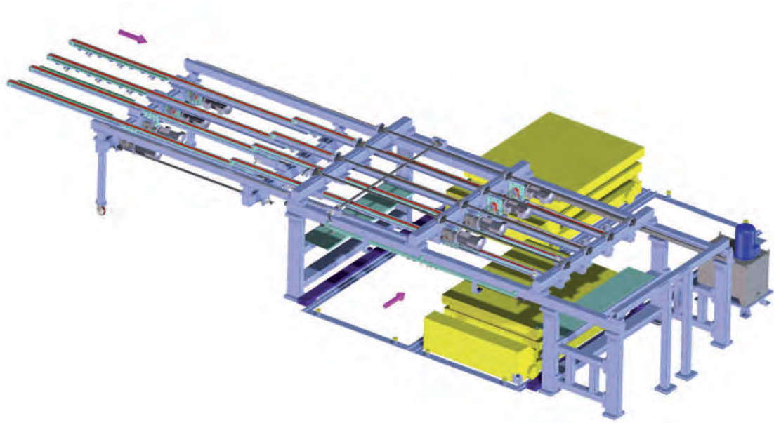
MAGNETIC STACKER
